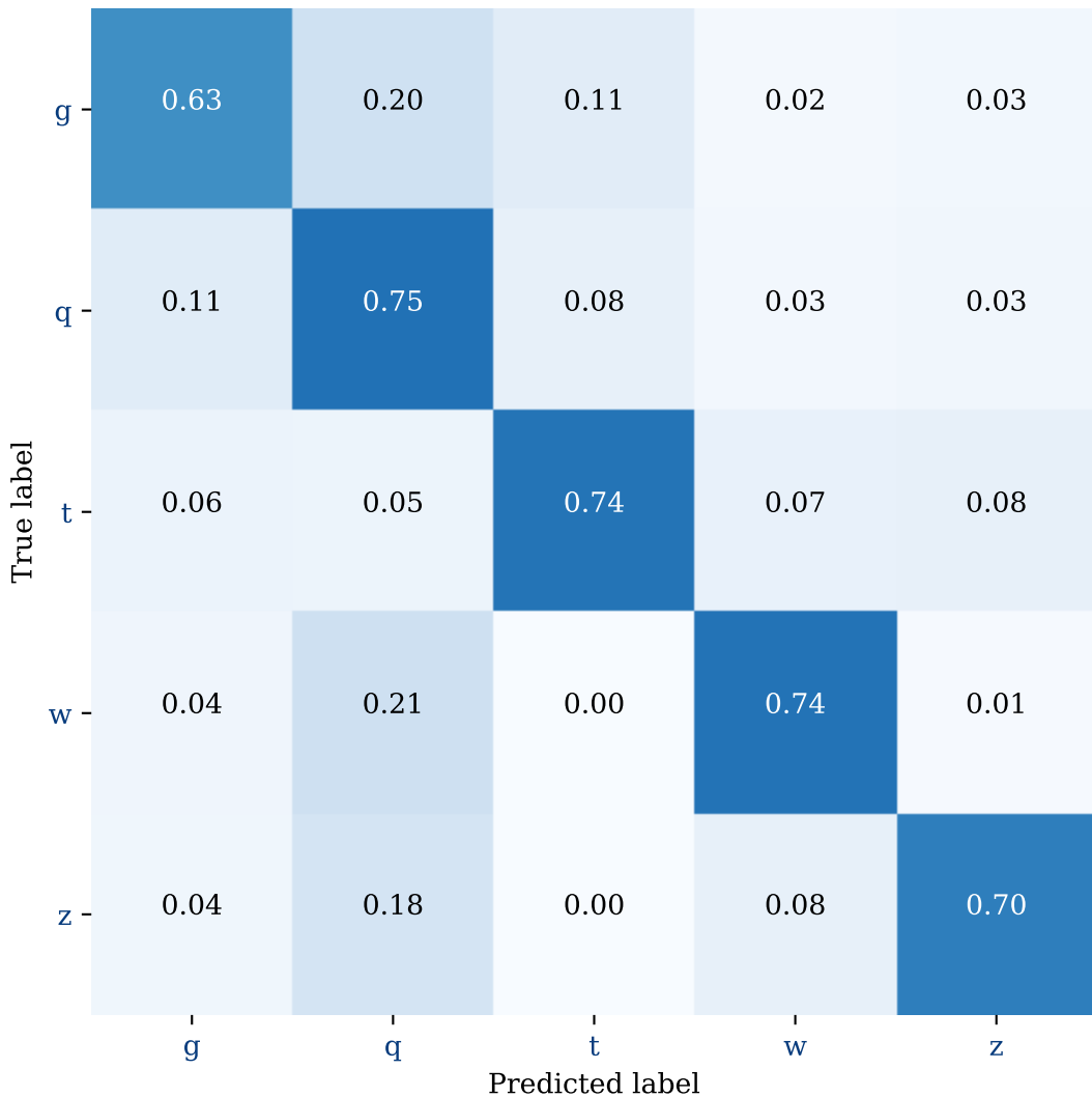
Confusion Matrix of Jet-tagger: HGQ with 303 EBOPs
